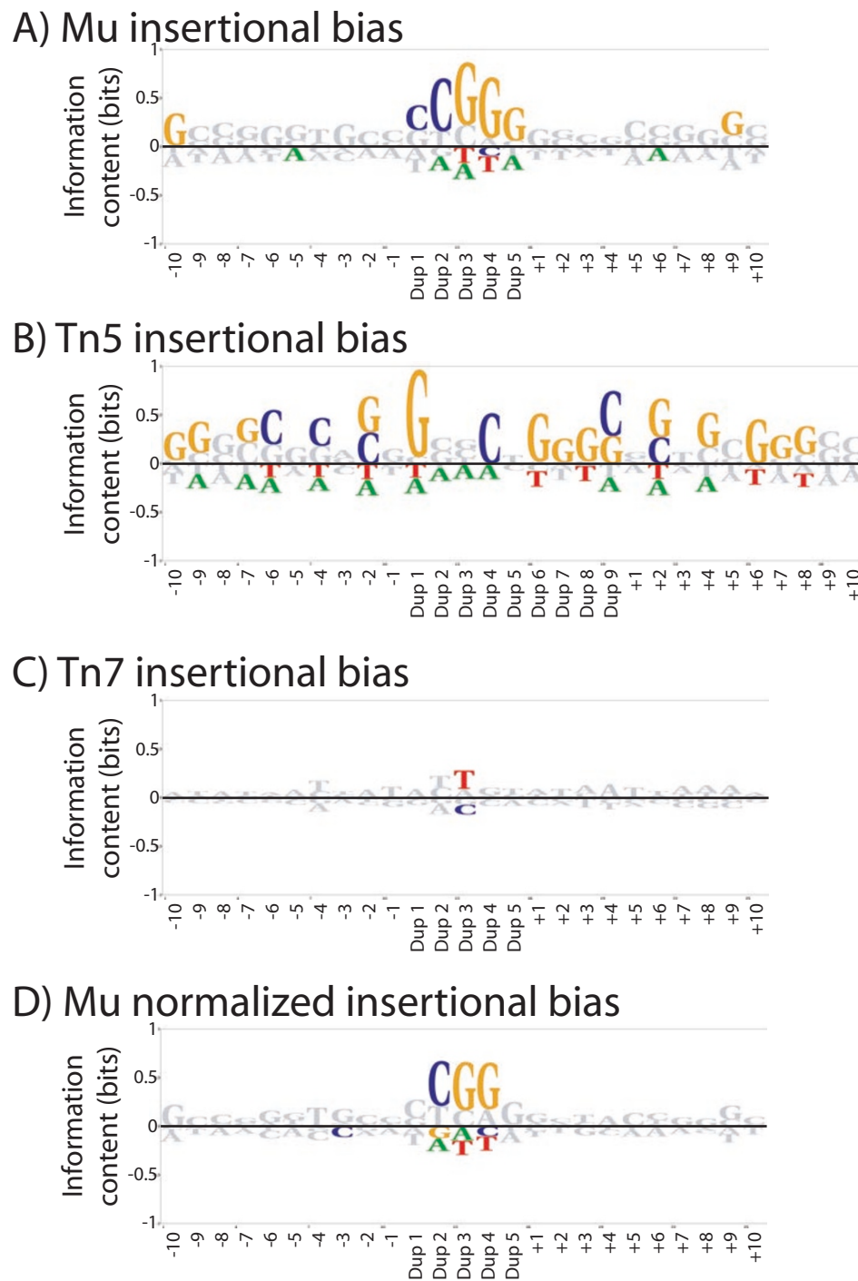
Figure 1 Insertion biases of Mu, Tn5, and Tn7. BLogo sequence logos are shown for all insertion sites for Mu (A), Tn5 (B), and Tn7 (C) transposons into Candida glabrata subtelomeric DNA. Ten bases on either side of the transposon mediated duplication of five (Mu and Tn7) or nine (Tn5) bases were used to generate the sequence logo, and bases significant at P < 0.001 are shown in color. Mu insertion events were used to create a BLogo sequence logo with background base frequencies obtained from selecting all 25 mers within the target fosmids containing a central CGG (D). The background frequencies of A, C, G, and T used for the BLogo sequence logos are respectively: 0.32, 0.19, 0.18, 0.31 (A,B,C); 0.275, 0.217, 0.224, 0.284 (D).
